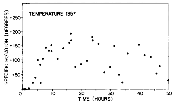
Figure 2. Specific rotations produced at 135° in polycrystalline samples of 1,1'-binaphthyl taken from an ordinarily prepared racemic sample.
